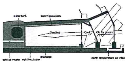
Earthship with two bufferzones
